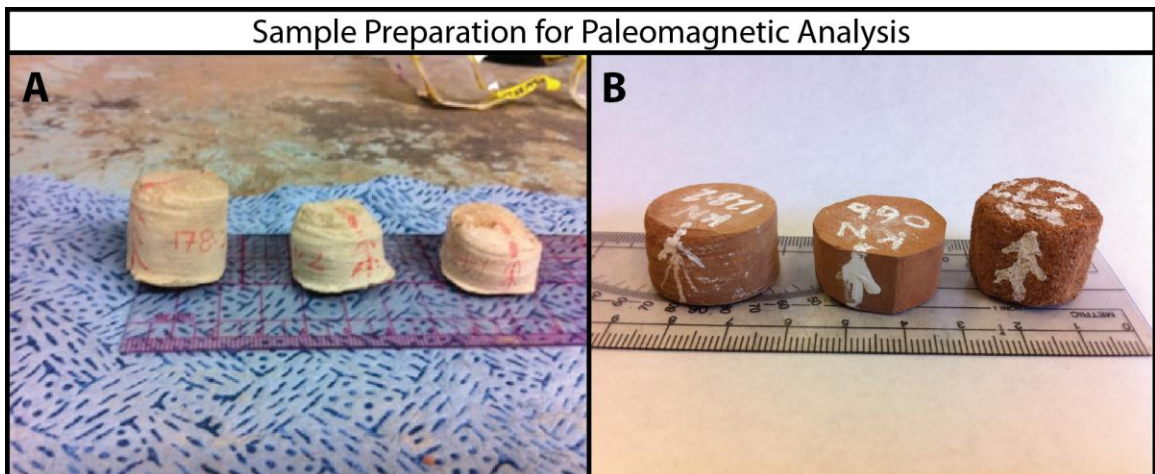
Figure A2 - Core sample preparation for paleomagnetism analysis. A) Raw samples from the field. B) Samples that have been filed to size and relabeled, ready for analysis.
