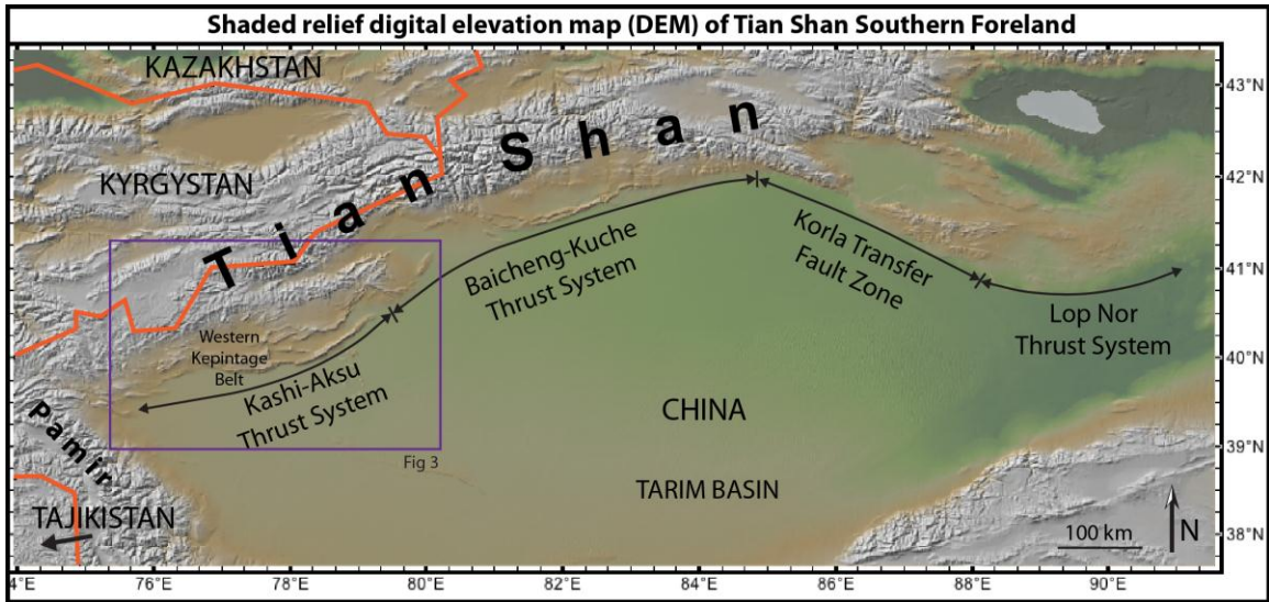
Figure 2 - Shaded relief digital elevation map showing the extent of the Tian Shan foreland. Orange lines represent country borders. Purple box indicates Figure 3. (DEM courtesy of geomapapp.org)
