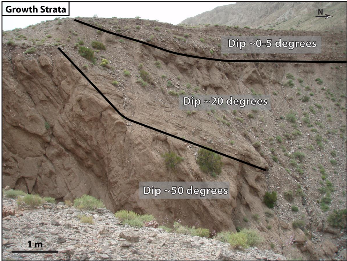
Figure 16 - Growth strata observed on the backlimb of the Southern Tashenkou fault-propagation fold near the North Kepintage Thrust Fault. Strata exhibit the characteristic fanning associated with growth strata. Growth strata is at the top of the Xiyu Conglomerate.
