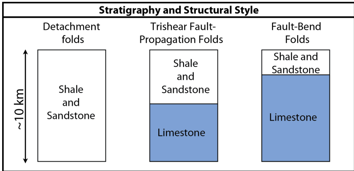
Figure 19 – Schematic of the relationship between stratigraphy and structural style. Where the strata above the décollement are dominated by relatively young (Neogene) sandstones and shales, detachment folds dominate as in the Kashi Basin (Heermance et al., 2008) and Aksu Re-entrant (Hubert-Ferrari et al., 2005). Where the strata above the décollement are approximately half relatively young (Neogene) sandstones and shales and half old (Paleozoic) limestone and other shallow marine sediments, fault-propagation folds with a trishear component dominate as in Medial Tashenkou and Southern Tashenkou regions (this study). Where the strata above the décollement are approximately a quarter relatively young (Neogene) sandstones and shales and three quarters old (Paleozoic) limestone and other shallow marine sediments, fault-bend folds dominate as in Northern Tashenkou region (this study).
