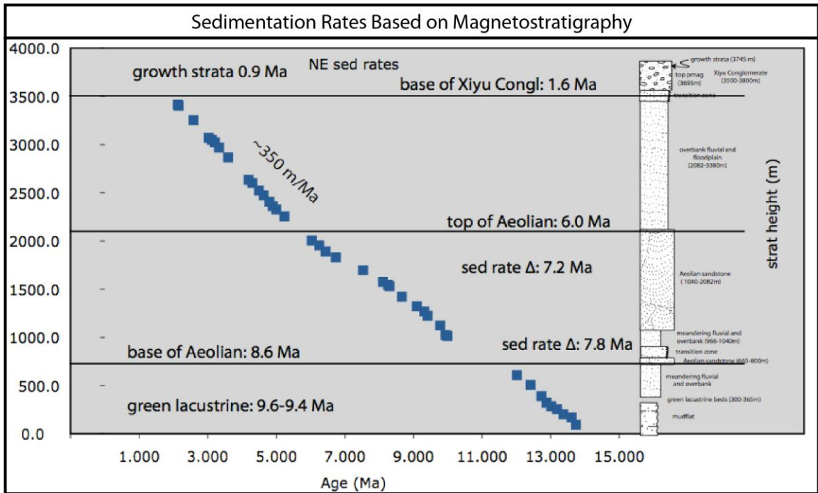
Figure A4 - Sedimentation rates using Alternative correlation A from the magnetostratigraphy. Sedimentation rates are 350 m/Ma, with an increase in sedimentation rate to 1000 m/Ma between 7.8 and 7.2 Ma.
