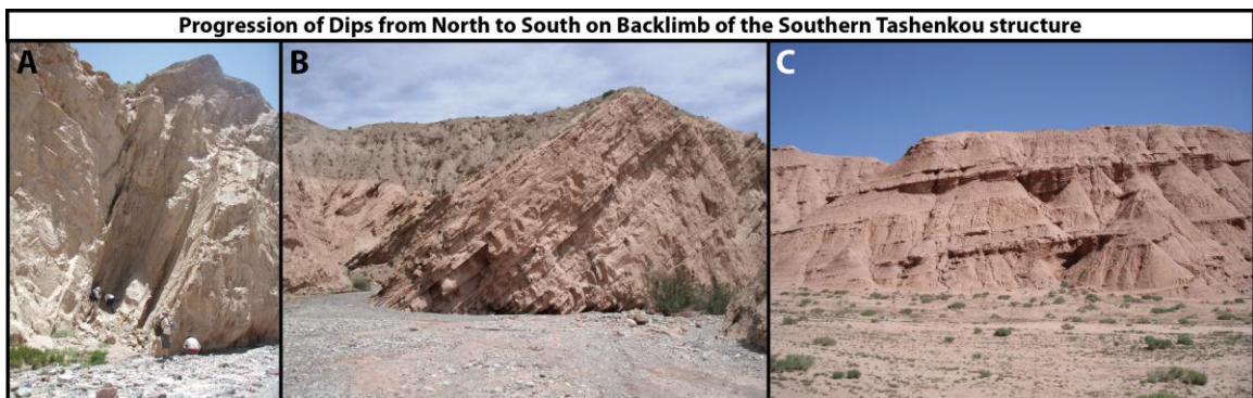
Figure 14 – Southern Tashenkou region progression of dips of Neogene strata between the North Kepintage Thrust Fault and the crest of the Southern Tashenkou structure. A) strata are dipping approximately 65° degrees to the north, B) strata are dipping approximately 40° degrees to the north, C) strata are dipping approximately 10° to the north.
