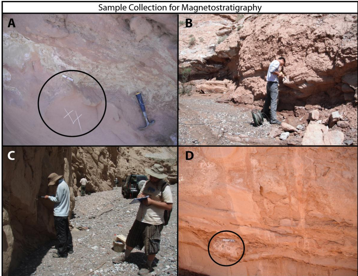
Figure A1 - Sampling for magnetostratigraphy. A) Mark location of sample on strata with X and nail ID tag to strata. B) Drill sample core from strata. C) Measure orientation of core sample in situ and record dip of strata. D) Core samples removed from strata.
