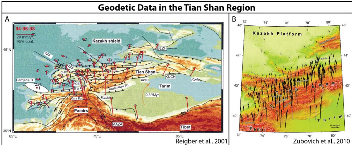
Figure 6 – Geodetic data in the Tian Shan region. A) Geodetic data from Reigber et al., 2001. Geodetic data suggests a shortening rate of 8 \pm 3 mm/yr. B) Geodetic data from Zubovich et al., 2010. Geodetic data suggests a shortening rate of 4-7 mm/yr.
