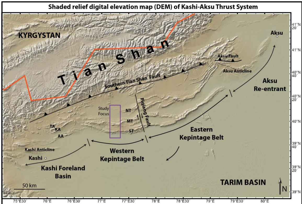
Figure 3 - Shaded relief digital elevation map of the Kashi-Aksu Thrust System. Orange line represents country borders. Main cities (Kashi and Aksu) of the Kashi-Aksu Thrust System are shown. Piqaing Fault divides the western and eastern segments of the Kepintage belt. TA – Tashipishake Anticline, KA – Keketamu Anticline, AA – Atushi Anticline, NT – Northern Tashenkou region, MT – Medial Tashenkou region, ST – Southern Tashenkou region. (DEM courtesy of geomapp.org)
