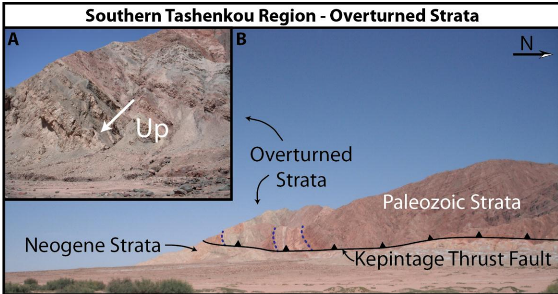
Figure 13 – Southern Tashenkou region. A) Overturned strata near the Kepintage Thrust Fault. B) Paleozoic strata thrust over Neogene strata; overturned strata delineated with blue dashed lines.
