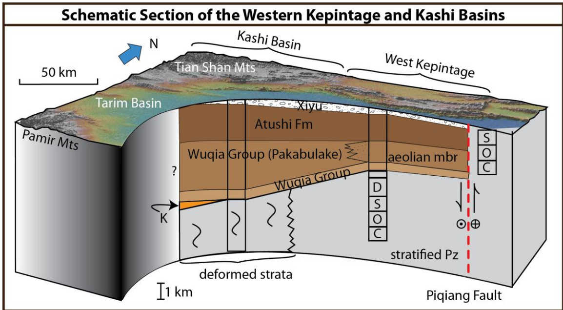
Figure 18 - Schematic section of the western Kepintage and Kashi Basins. This figure illustrates the correlation of strata across the segments, as well as the change in stratigraphic thickness across the segments and the Piqiang Fault.
