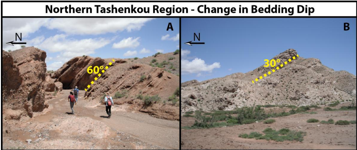
Figure 11 – Northern Tashenkou Region. A) Bedding is dipping approximately 60°-70° to the north. B) Bedding is dipping approximately 30° to the north. Location A is approximately 1 km north of location B.
