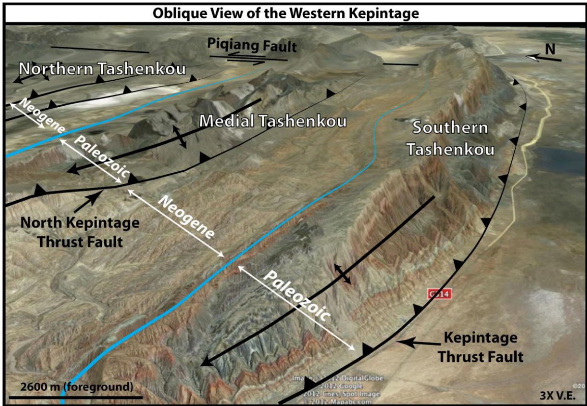
Figure 4 - Oblique view of the western Kepintage. Three main structures identified, and extent of Paleozoic and Neogene strata shown. Blue lines indicate boundary between each region. (map courtesy of Google Earth)
