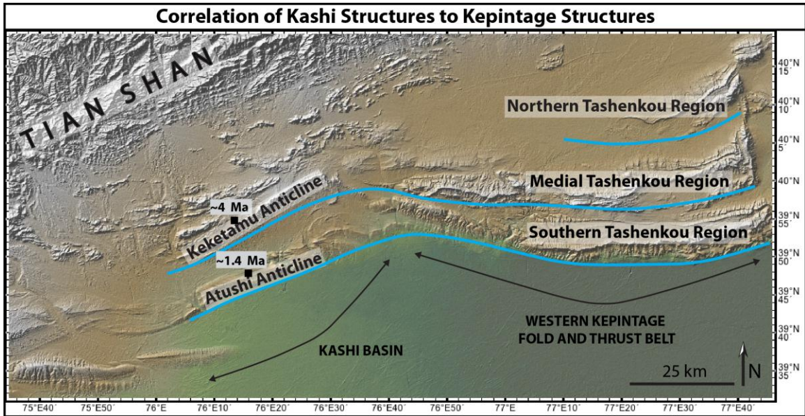
Figure 17 - Shaded relief digital elevation map of the western Kepintage and Kashi basin. Medial Tashenkou and Southern Tashenkou regions are correlative to the Keketamu and Atushi Anticlines, respectively. Ages in Kashi Basin from growth strata and magnetostratigraphy (Heermance et al., 2007).
