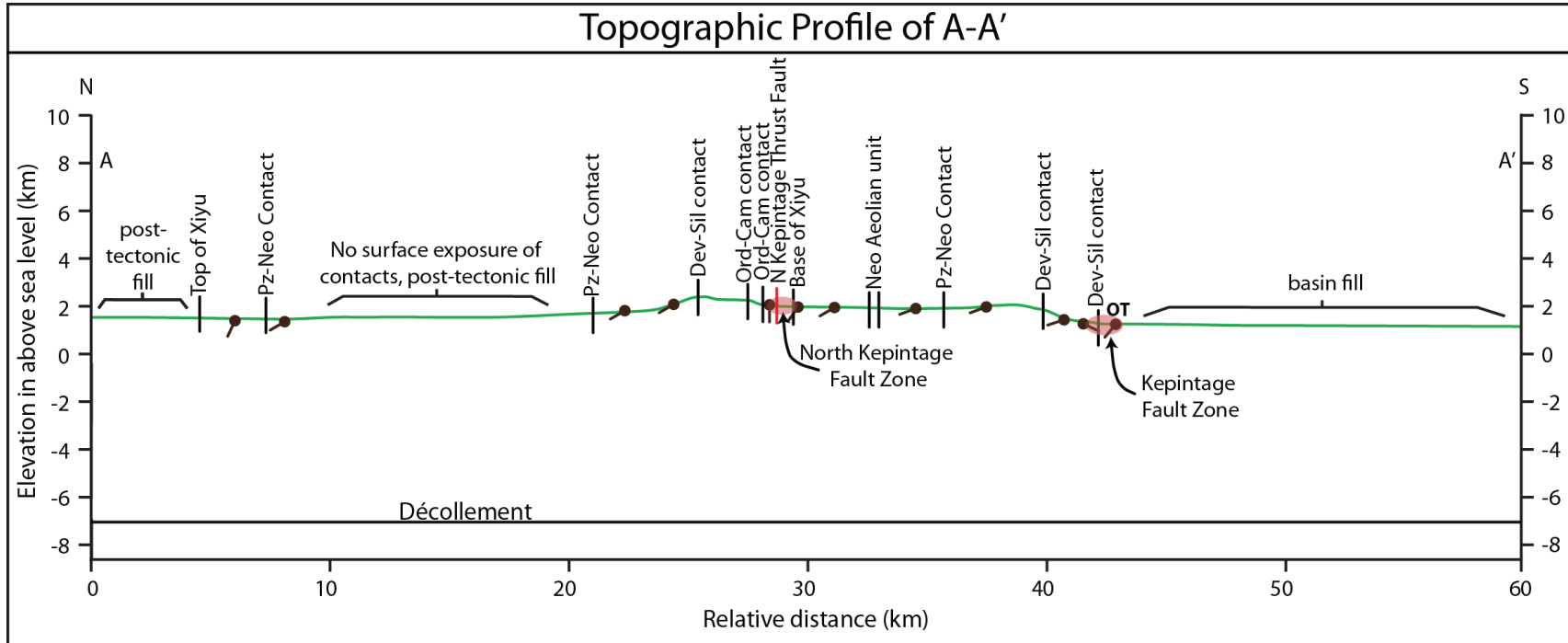
Figure 8 – Topographic profile of A-A' illustrating dip data, fault locations, stratigraphic contacts, and depth to décollement. Green line is the topographic profile from A to A', black tick marks are stratigraphic contacts, red tick is discrete fault, red ovals are fault zones.
