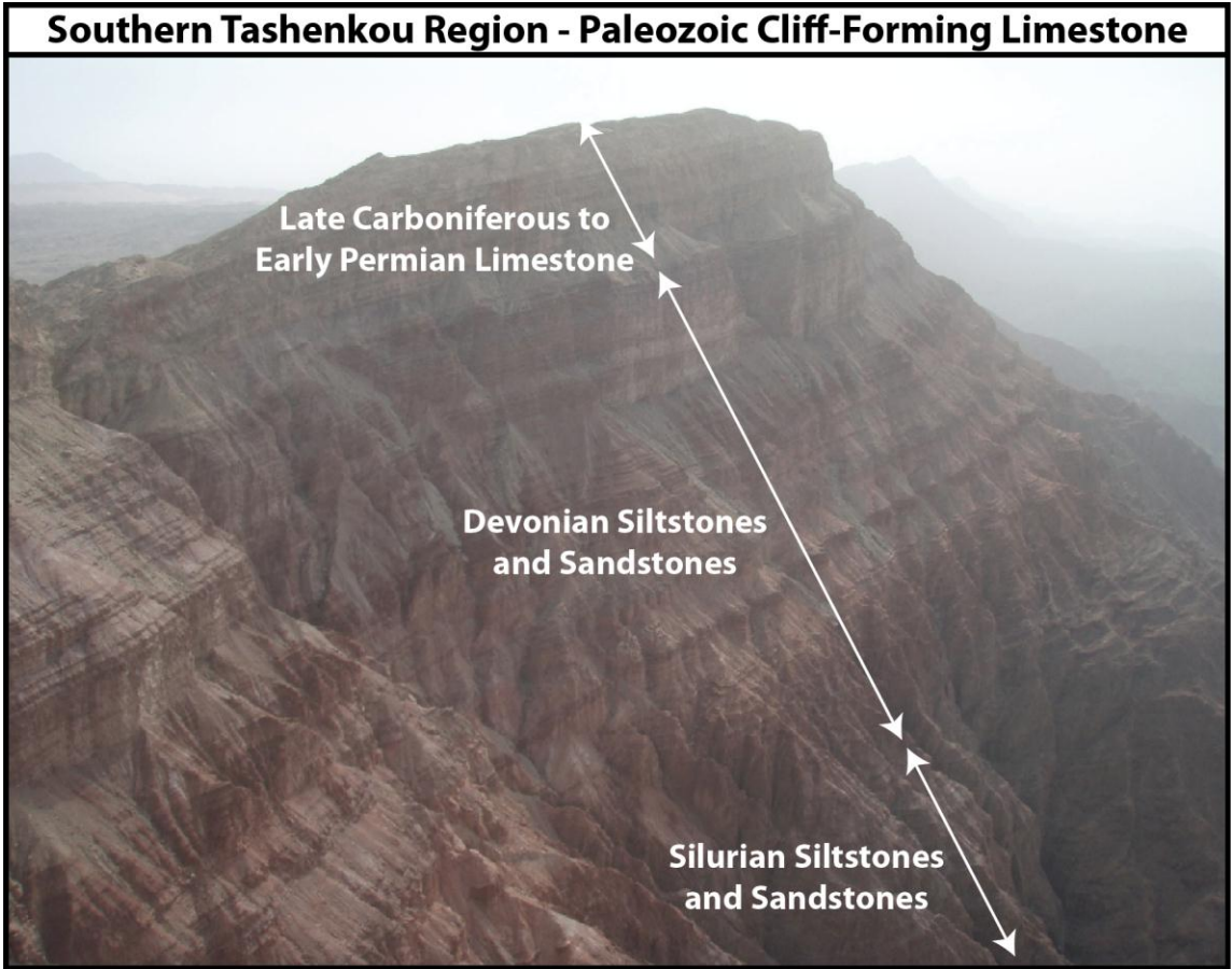
Figure 21 – Paleozoic limestone is the cliff-forming strata in the western Kepintage.
