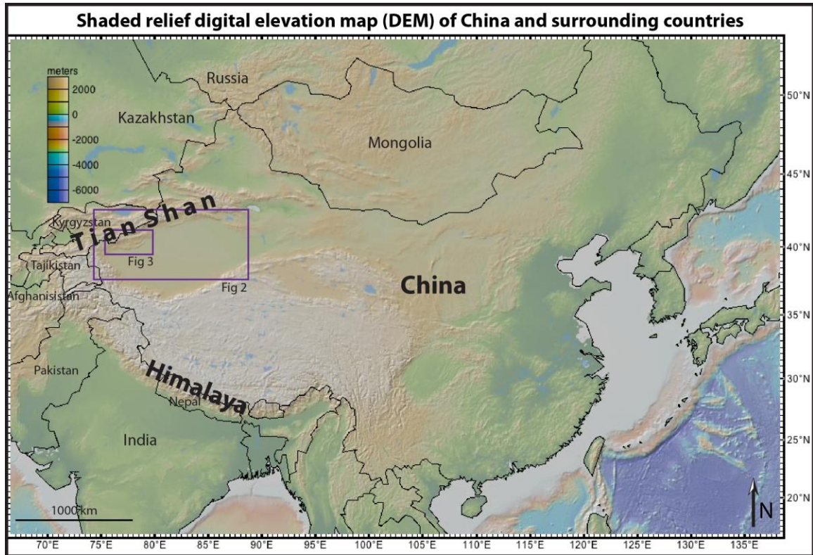
Figure 1 - Shaded relief digital elevation map indicating the area of interest, the Kashi-Aksu thrust system of the Tian Shan foreland in northwestern China. The Tian Shan and Himalaya Ranges are shown. Black lines represent country borders. Purple boxes indicate Figure 2 and Figure 3. (DEM courtesy of geomapapp.org)
