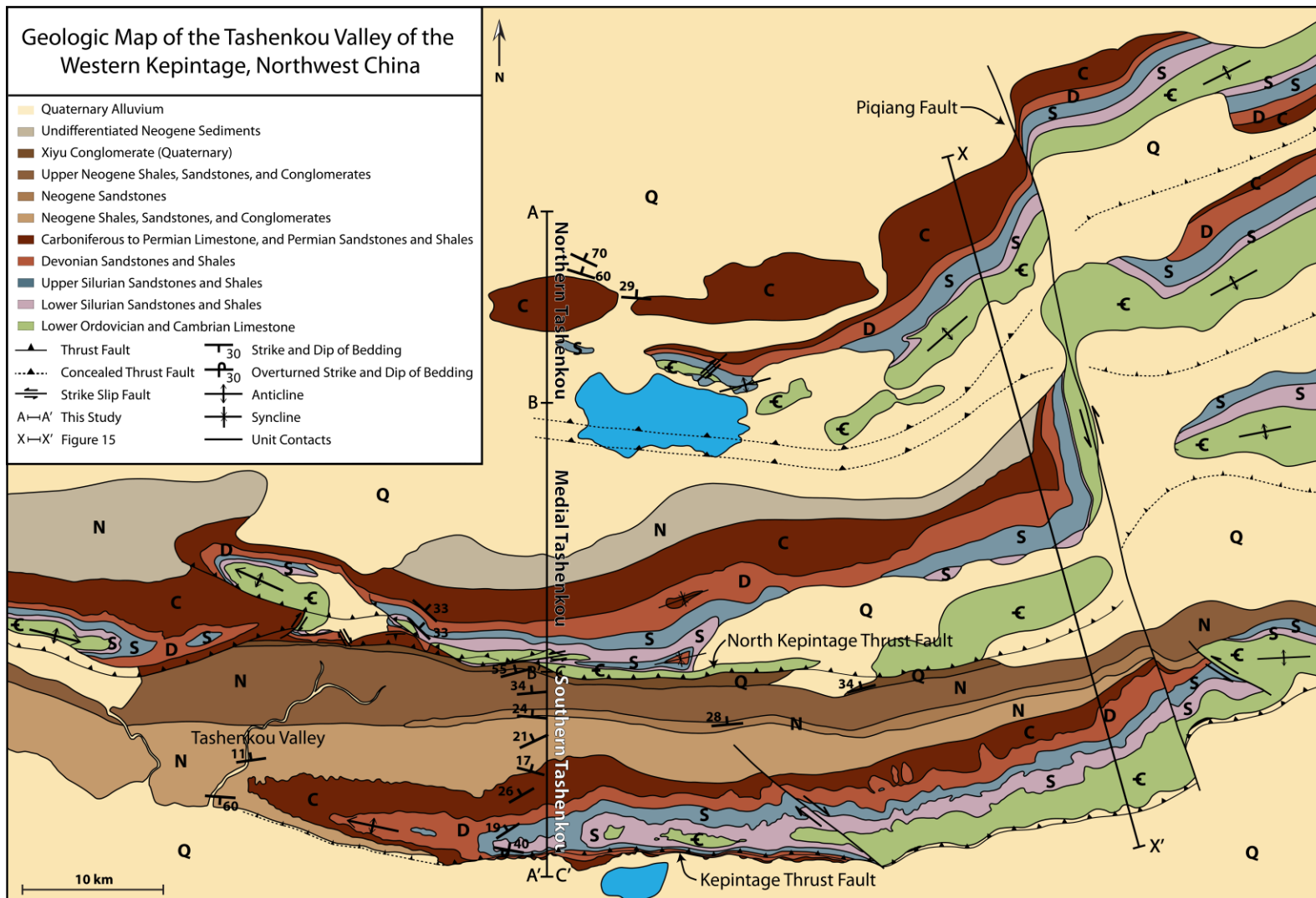
Figure 5 - Geologic map of the western Kepintage. Regions named for the Tashenkou river drainage.
