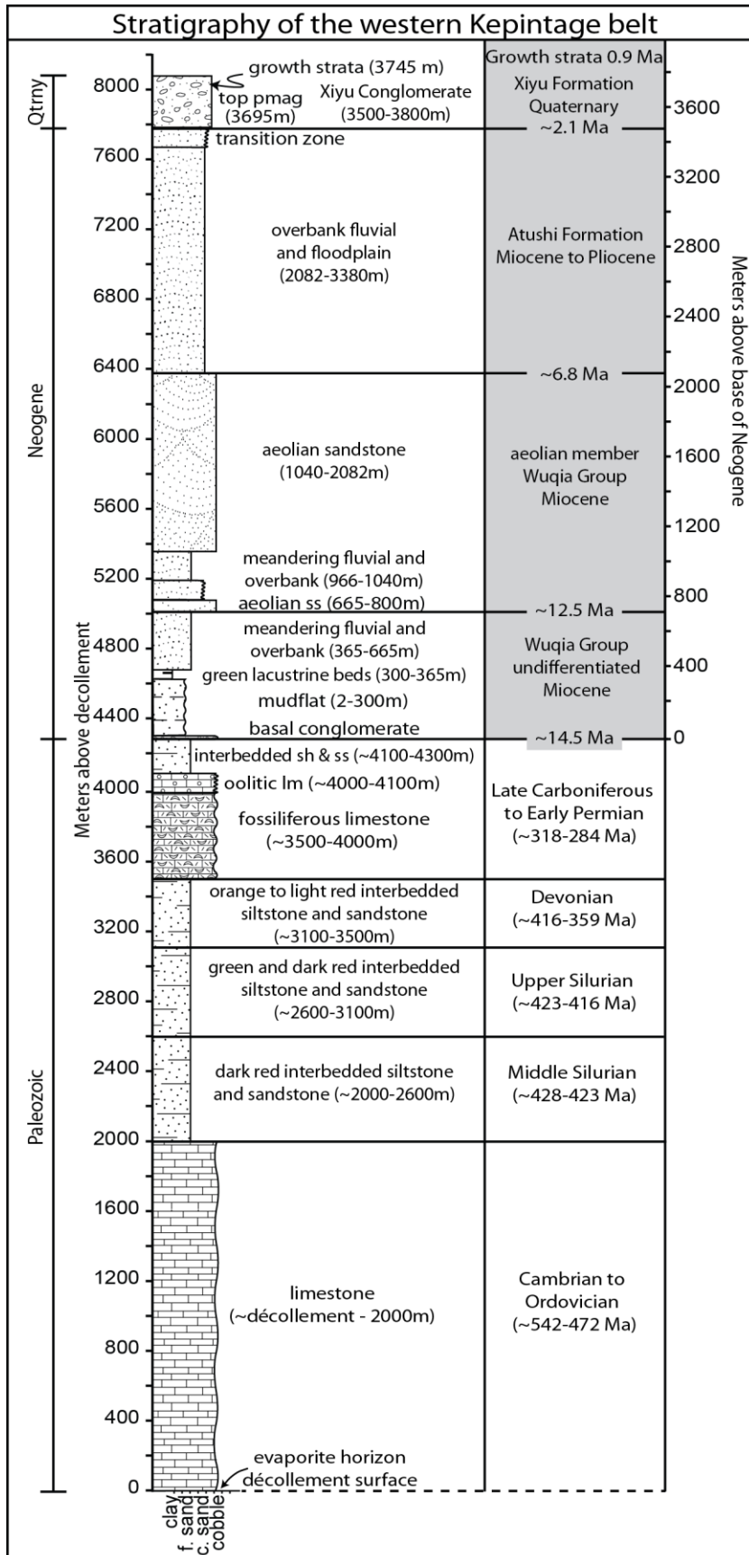
Figure 9 - Composite stratigraphic column of the western Kepintage fold and thrust belt. Depths, thickness, and description of Paleozoic stratigraphy are based on field strike and dip measurements, calculated thicknesses, and previously published literature. Neogene stratigraphy was measured in the field with a Jacob Staff and Abney Level. Neogene ages are from correlation of stratigraphy in the western Kepintage to the Kashi Basin. Scale on the left is the approximate measured stratigraphic height above décollement. Scale to the right is measured height above Neogene-Paleozoic contact.
