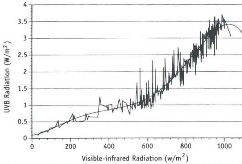
FIGURE 3. The 5th-order polynomial regression between UVB and visible-infrared radiation in 1996 at Northridge.
