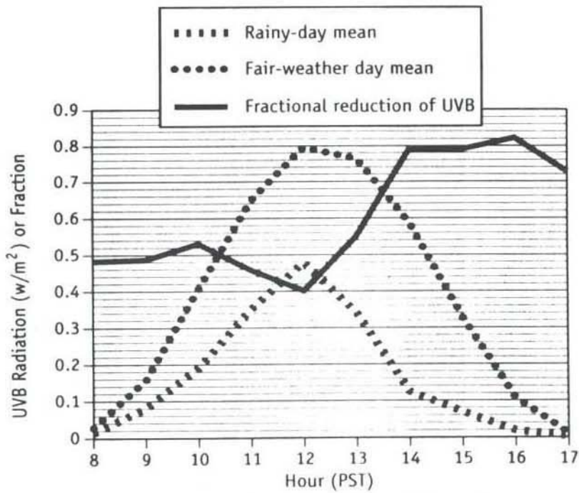
FIGURE 4. Mean hourly UVB radiation on rainy and fair-weather days and the fractional reduction of UVB radiation on rainy days in December 1996 at Northridge.
