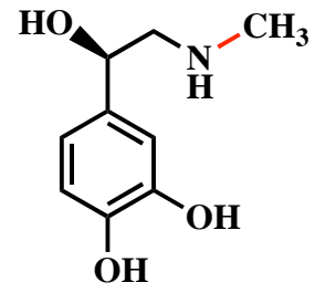
epinephrine
