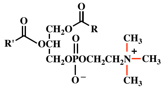
phosphatidylcholine
