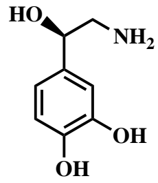
norepinephrine
