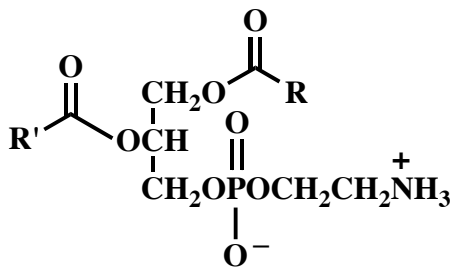
phosphatidylethanolamine
