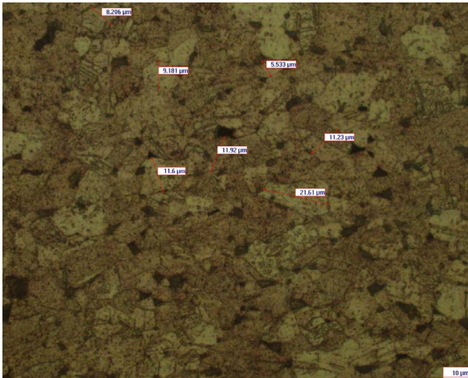
Brass - 600C - 50X
